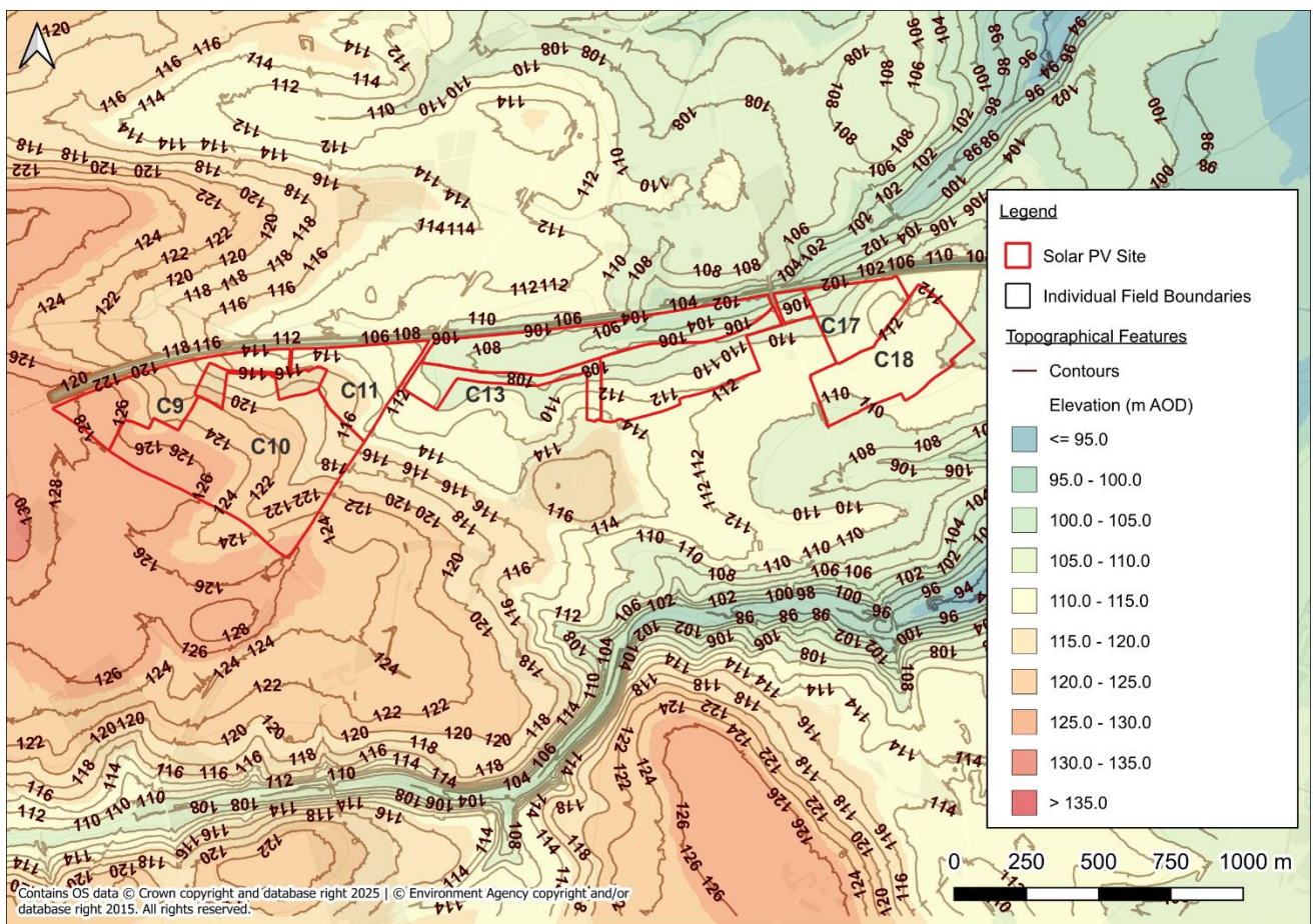
Figure 2: LiDAR Plan
